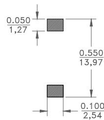
LAND PATTERN
