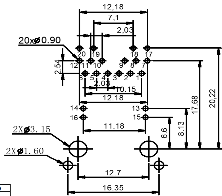
COMPONENT SIDE VIEW LANDED PATTERN
